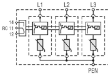
ETITEC T2 3+0 RC
