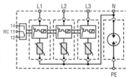
ETITEC T2 3+1 RC
