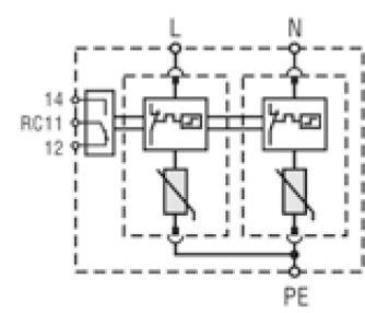
ETITEC T2 2+0 RC
